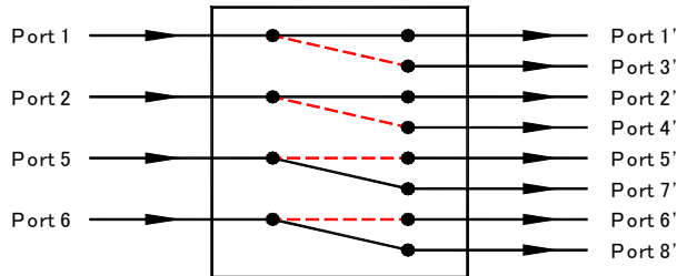
LB Quad 1x2 Bypass MM Switch
